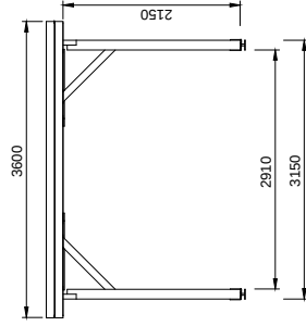
FRONT 1:100
